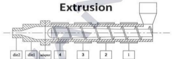
Type: screw: 45mm, L/D: 30, compression ratio 3:1
